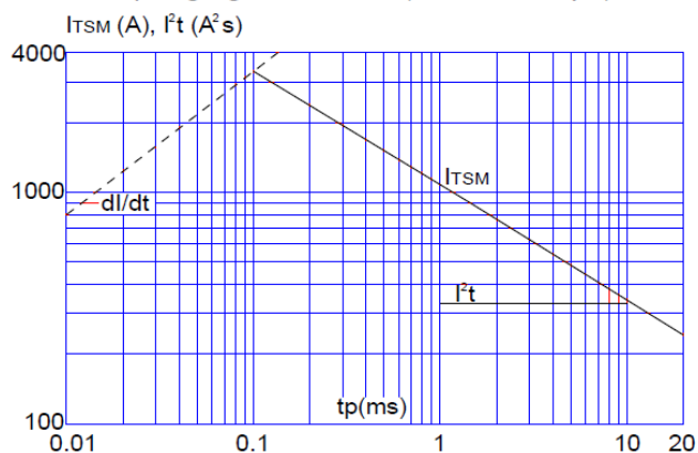
FIG.5: Non-repetitive surge peak on-state current for a sinusoidal pulse with width tp<10ms, and corresponding value of I²t (di/dt < 50A/µs)
