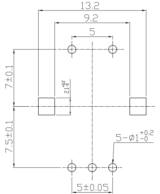
P.C.B.MOUNTING DETAIL
