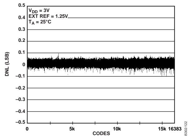
Figure 23. DNL AD5648-1
