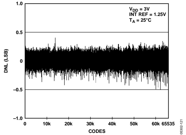
Figure 22. DNL AD5668-1
