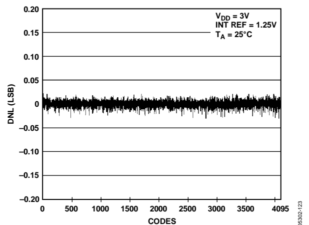
Figure 24. DNL AD5628-1
