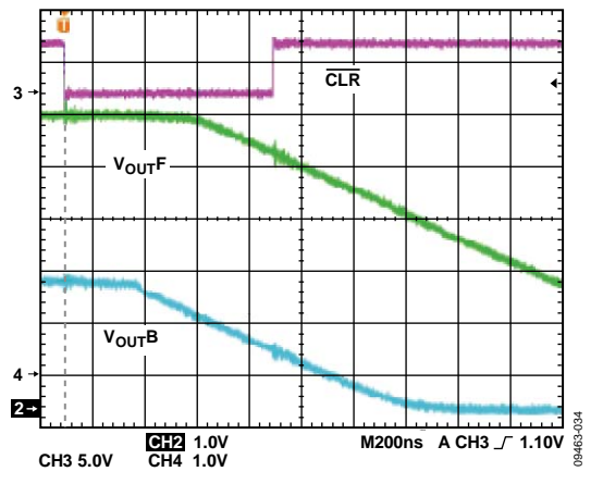
Figure 33. Hardware CLR
