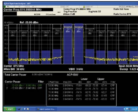
Figure 26. Two-Carrier W-CDMA at 875 MHz
