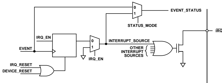
Figure 174. Simplified Schematic of \overline{\text{IRQ}} Circuitry
