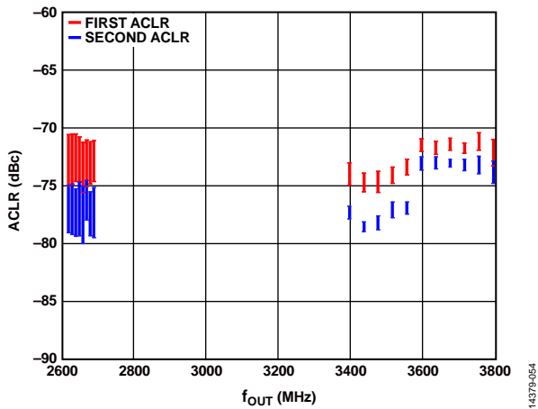
Figure 106. Single-Carrier, W-CDMA ACLR vs. f_{OUT} (First ACLR, Second ACLR)
