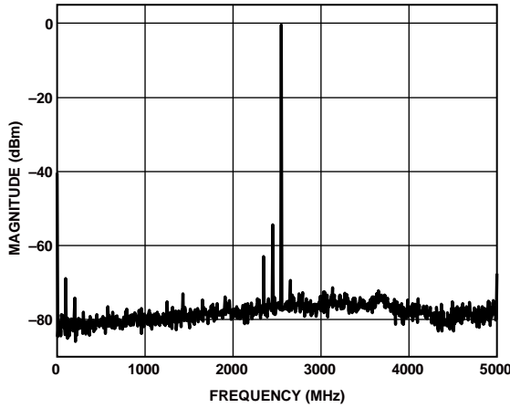
Figure 94. Single-Tone Spectrum at f_{OUT} = 2350 \text{ MHz} (FIR85 Enabled)
