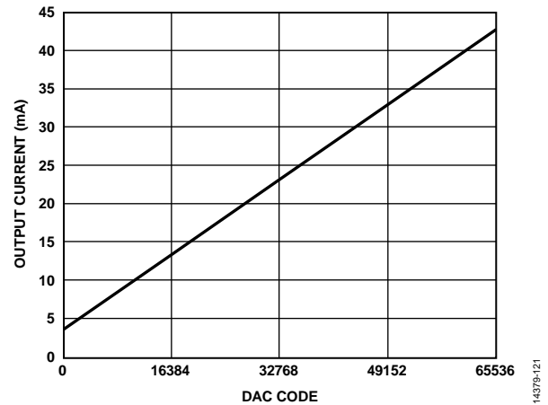
Figure 189. Gain Curve for ANA_FULL_SCALE_CURRENT[9:0] = 1023, DAC Offset = 3.8 mA
