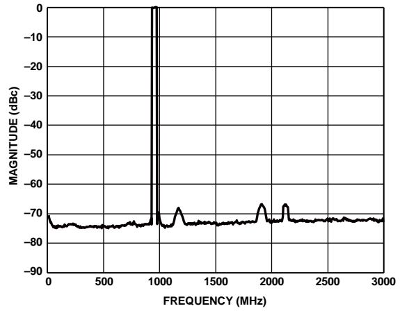
Figure 121. Eight Carriers at 950 MHz Output
