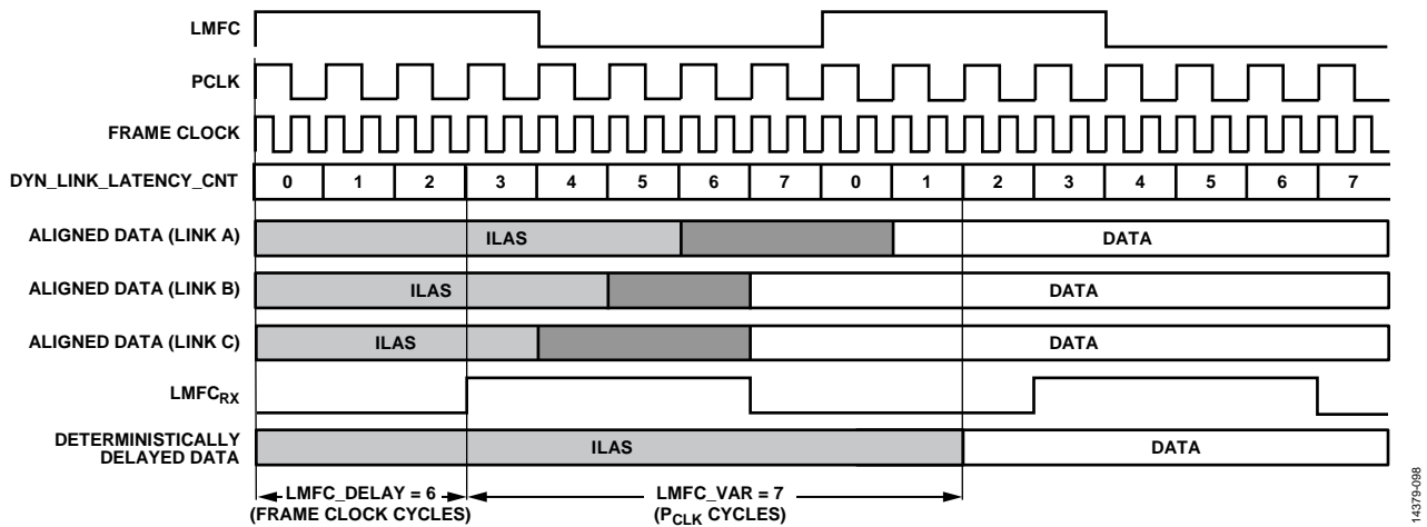
Figure 158. Multilink Synchronization Settings, Derived Method Example
