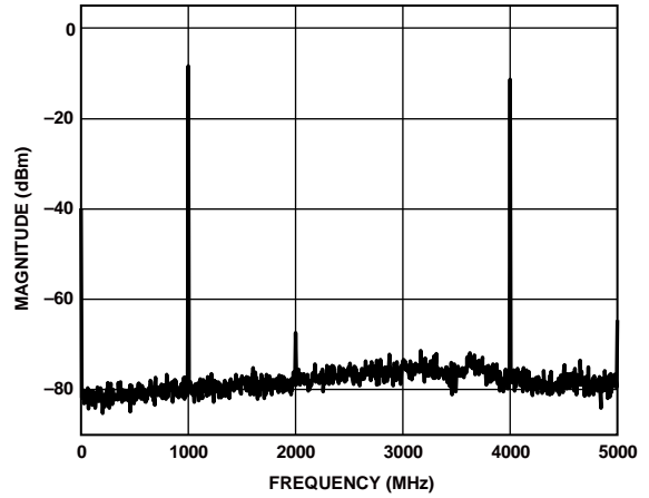
Figure 96. Single-Tone Spectrum at f_{OUT} = 4000 \text{ MHz}
