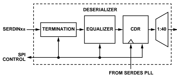
Figure 143. Deserializer Block Diagram
