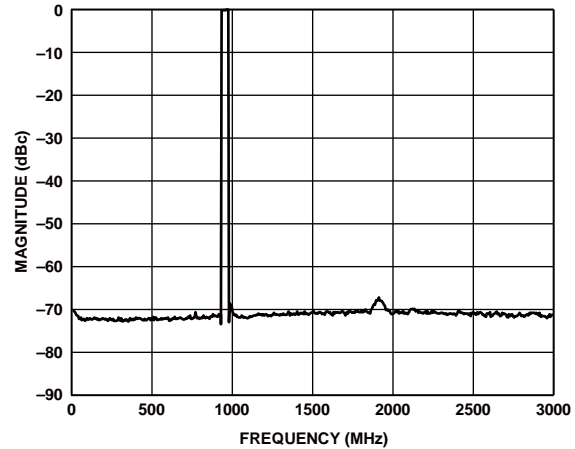
Figure 122. Eight Carriers at 950 MHz Output (Shuffle On)
