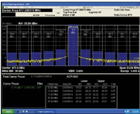
Figure 24. Single-Carrier W-CDMA at 877.5 MHz
