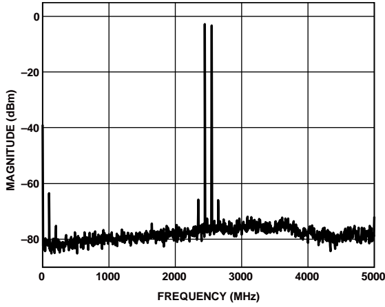
Figure 93. Single-Tone Spectrum at f_{OUT} = 2350 \text{ MHz}
