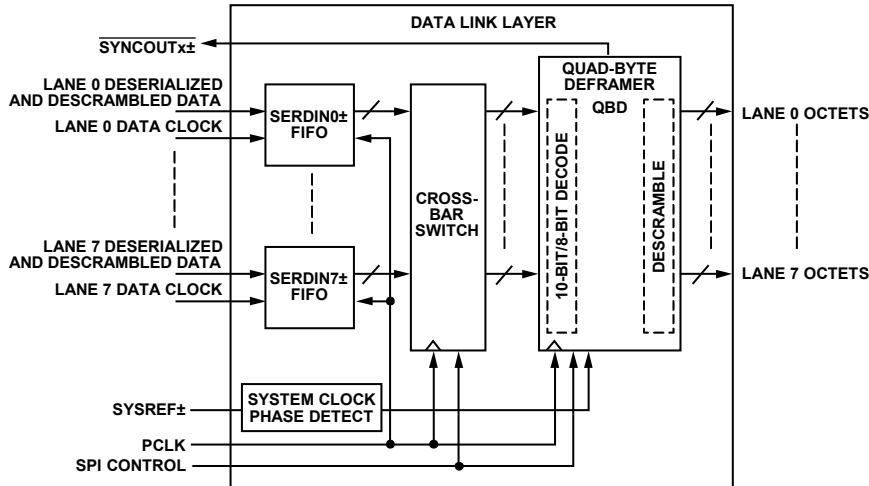
Figure 149. Data Link Layer Block Diagram
