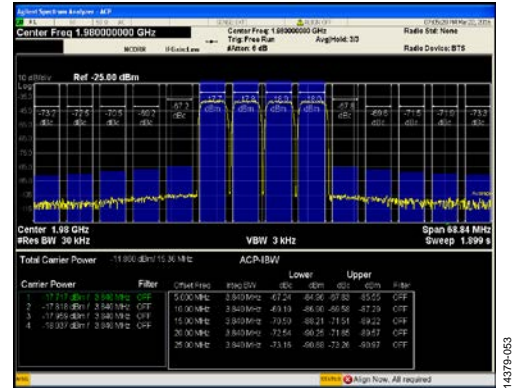
Figure 108. Four-Carrier W-CDMA at 1980 MHz
