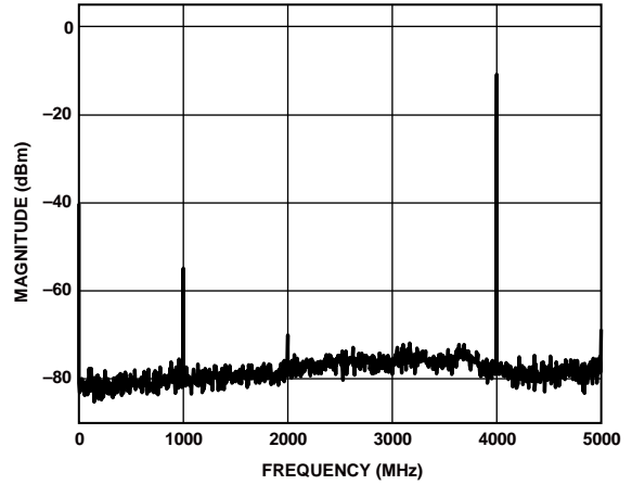
Figure 97. Single-Tone Spectrum at f_{OUT} = 4000 \text{ MHz} (FIR85 Enabled)
