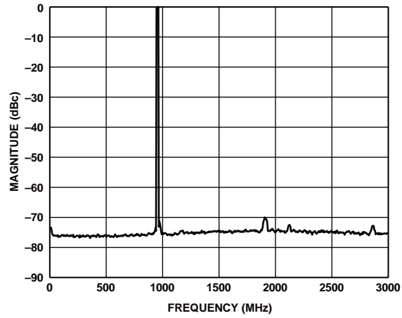
Figure 120. Four Carriers at 950 MHz Output (Shuffle On)
