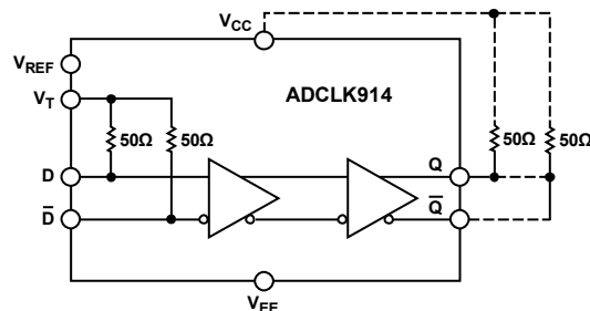
Figure 113. ADCLK914 Functional Block Diagram
