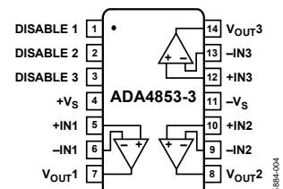
Figure 4. 14-Lead TSSOP
