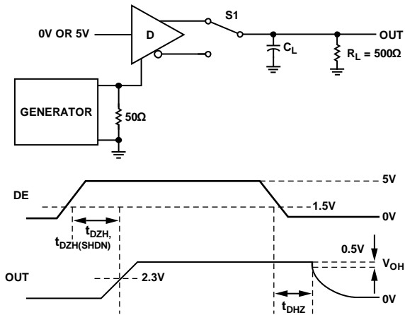
Figure 21. Driver Enable and Disable Times ( t_{DZH} , t_{DZH(SHDN)} , t_{DZL} , t_{DZL(SHDN)} )
