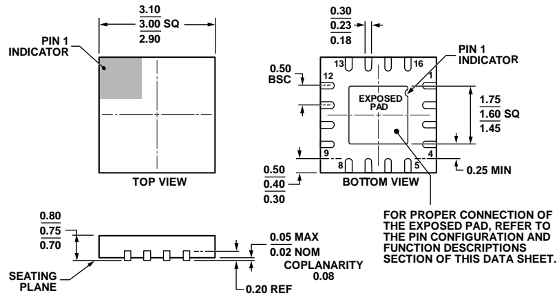
Figure 47. 16-Lead Lead Frame Chip Scale Package [LFCSP] 3 mm x 3 mm Body and 0.75 mm Package Height (CP-16-22) Dimensions shown in millimeters
