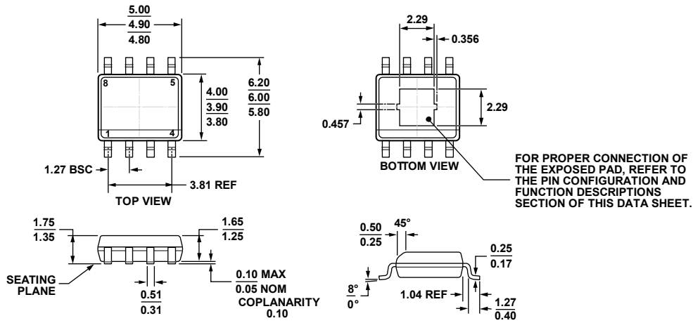
COMPLIANT TO JEDEC STANDARDS MS-012-AA Figure 64. 8-Lead Standard Small Outline Package, with Exposed Pad [SOIC_N_EP] Narrow Body (RD-8-1) Dimensions shown in millimeters
