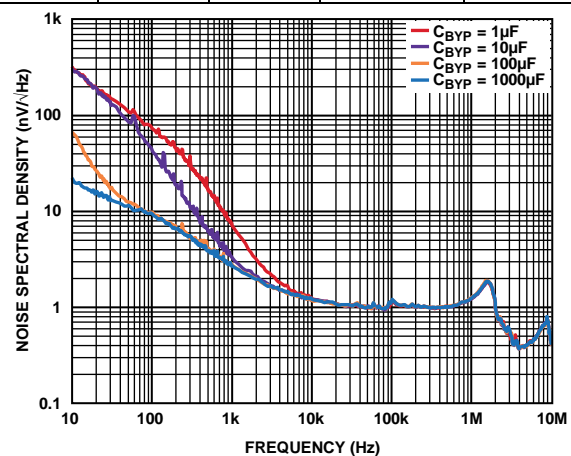
Figure 2. Noise Spectral Density at Different Values of C_{BYP} , V_{OUT} = 3.3 V
