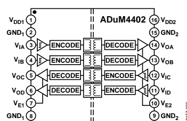
Figure 3. ADuM4402
