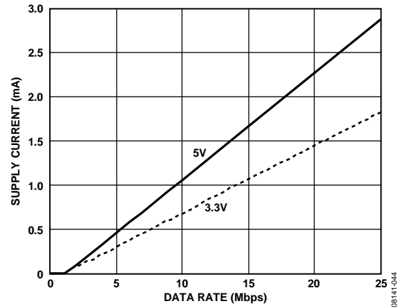
Figure 26. Typical I_{ISO(D)} Dynamic Supply Current per Output (15 pF Output Load)
