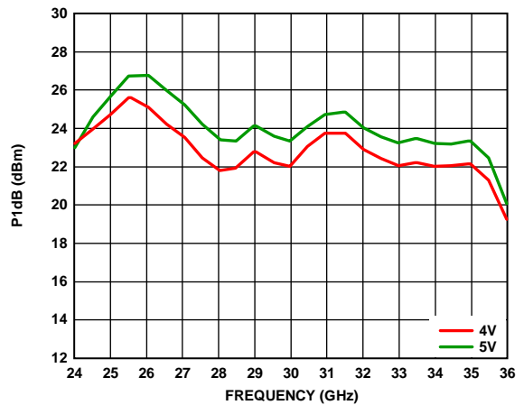
Figure 13. P1dB vs. Frequency at Various Supply Voltages
