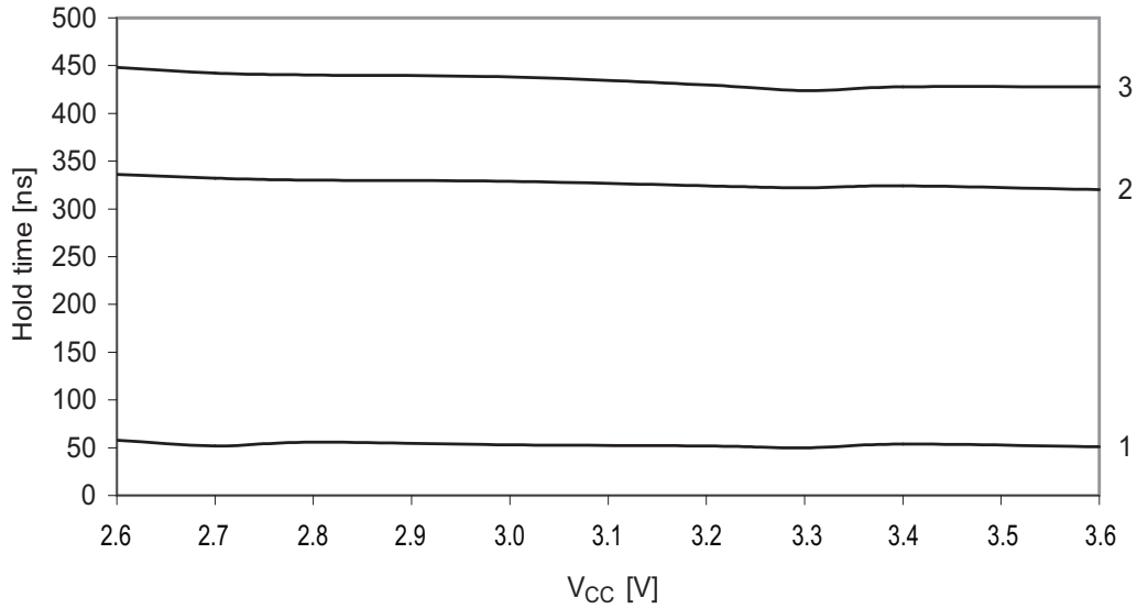
Figure 37-331. SDA hold time vs. supply voltage.
