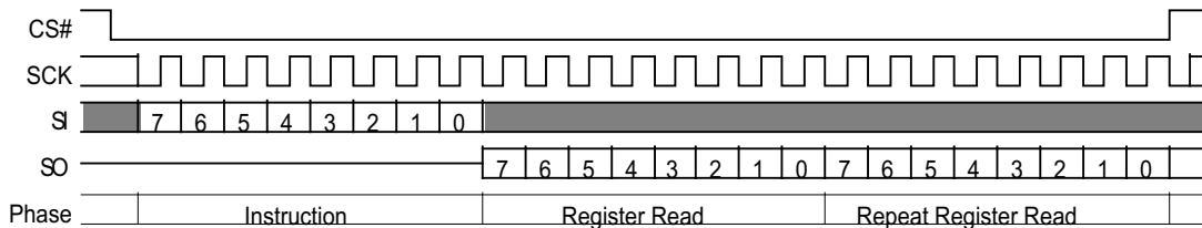
Figure 9.68 PPB Lock Register Read Command Sequence
