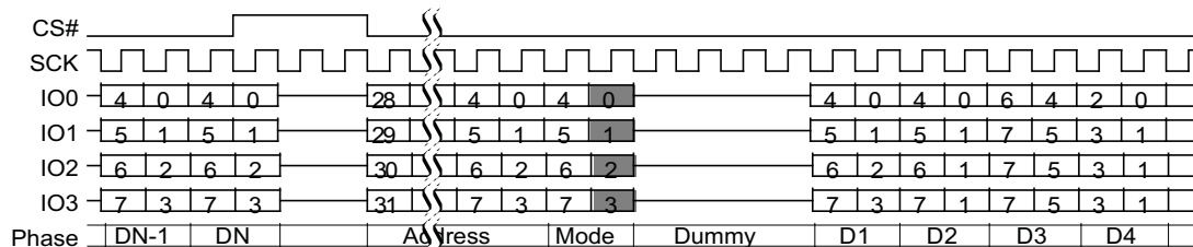
Figure 9.38 Continuous Quad I/O Read Command Sequence (4-Byte Address), LC=00b
