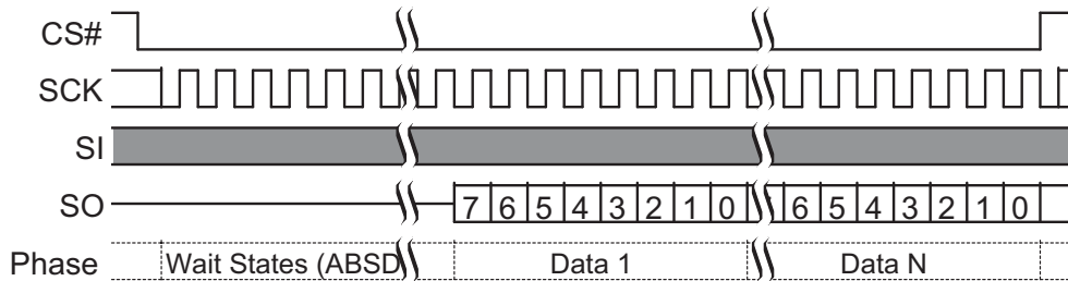
Figure 9.16 AutoBoot Sequence (CR1[1]=0)
