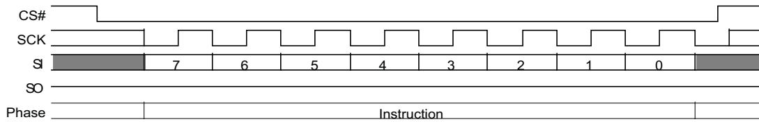
Figure 9.69 PPB Lock Bit Write (PLBWR A6h) Command Sequence
