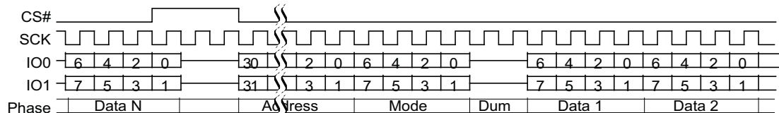
Figure 9.34 Continuous Dual I/O Read Command Sequence (4-Byte Address, BCh or BBh [ExtAdd=1], EHPLC=10b)
