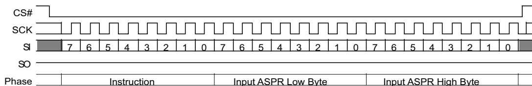
Figure 9.62 ASPP (2Fh) Command
