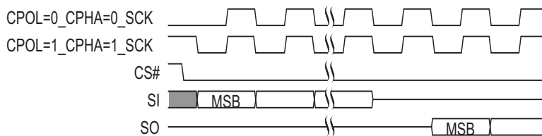
Figure 3.1 SPI SDR Modes Supported
