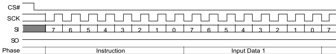
Figure 9.19 AutoBoot Register Write (ABWR) Command
