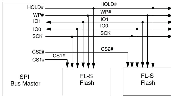
Figure 2.3 Bus Master and Memory Devices on the SPI Bus — Dual Bit Data Path
