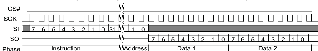
Figure 3.6 Single Bit Wide I/O Command without Latency
