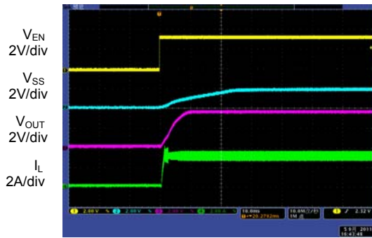
Time 10ms/div
