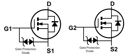
Equivalent Circuit
