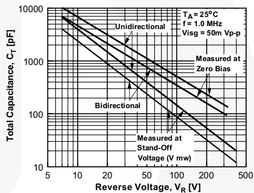
Figure 4. Total Capacitance
