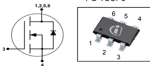
PG-TSOP6
