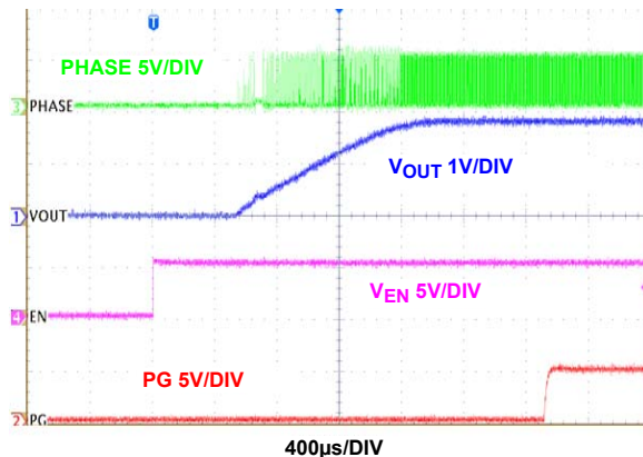
FIGURE 15. START-UP AT NO LOAD (PWM)
