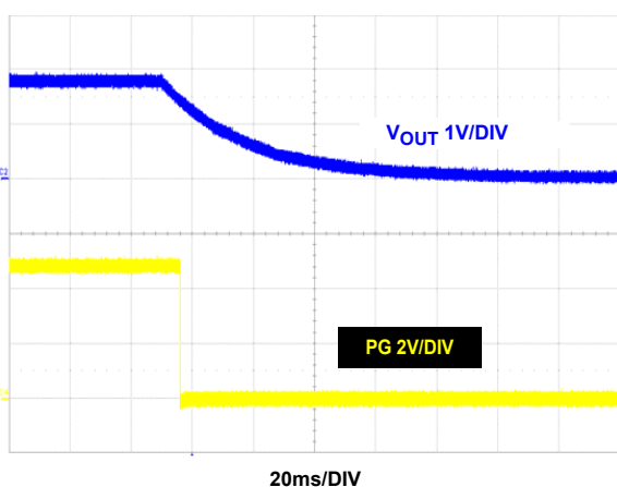
FIGURE 32. OVER-TEMPERATURE PROTECTION
