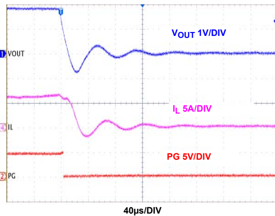
FIGURE 30. OVERCURRENT PROTECTION
