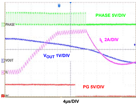
FIGURE 29. OUTPUT SHORT-CIRCUIT
