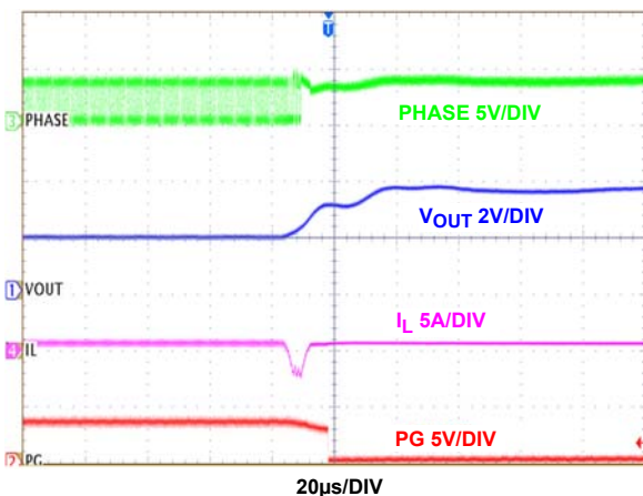
FIGURE 31. OVERVOLTAGE PROTECTION
