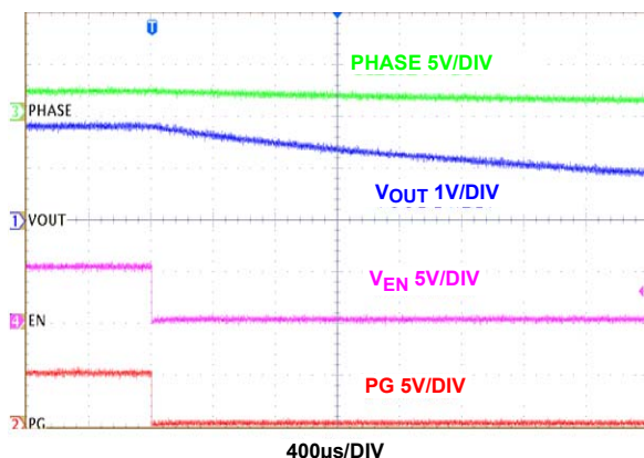
FIGURE 16. SHUTDOWN AT NO LOAD (PFM)
