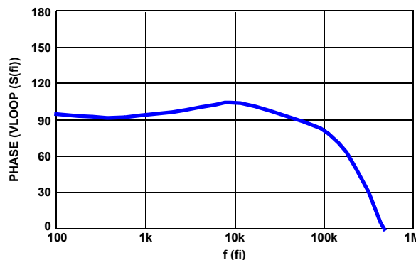
FIGURE 37. SIMULATED LOOP GAIN
