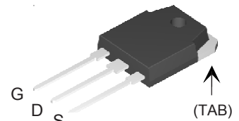
TO-3P (IXTQ)
