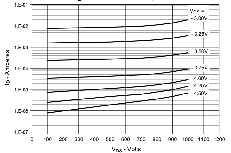
Fig. 4. Drain Current @ T_J = 25^\circ\text{C}
