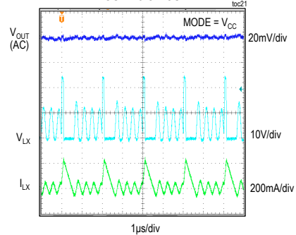
STEADY-STATE SWITCHING WAVEFORMS, 5V OUTPUT, DCM MODE, 25mA LOAD, FIGURE 3 CIRCUIT
