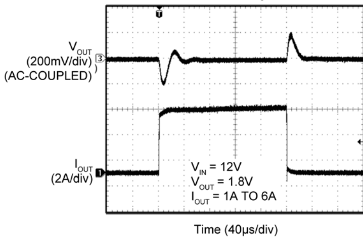
Transient Response
