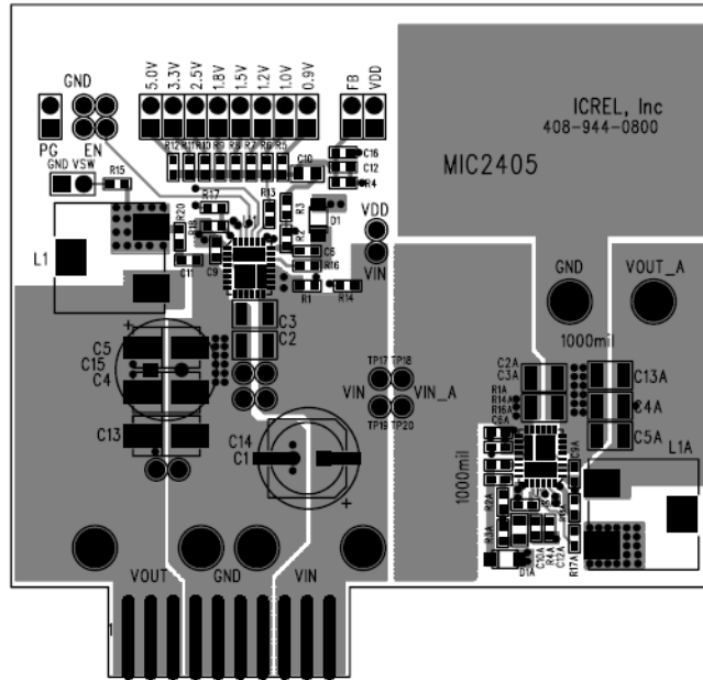
Figure 13. MIC24052 Evaluation Board Top Layer
