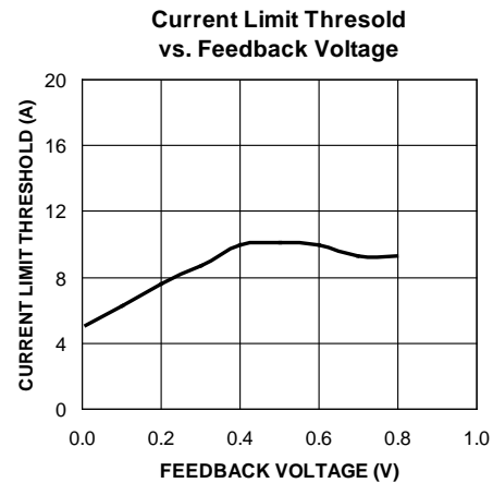
Figure 5. MIC24052 Current-Limit Foldback Characteristic
