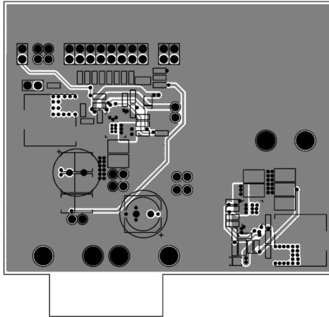
Figure 15. MIC24052 Evaluation Board Mid-Layer 2
