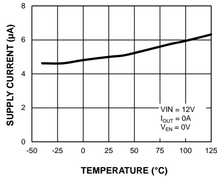
VIN Shutdown Current vs. Temperature
