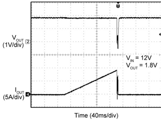
Output Current-Limit Threshold
