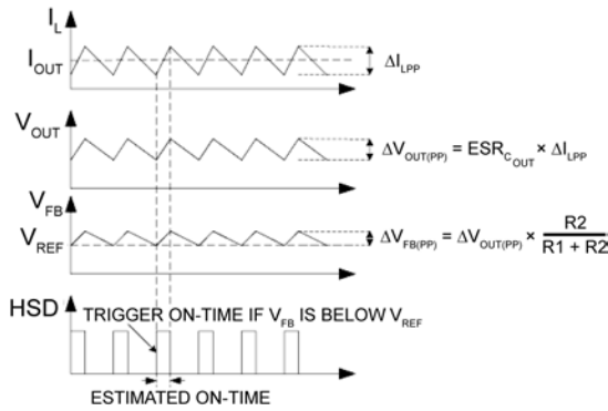
Figure 2. MIC24052 Control Loop Timing
