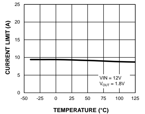
Output Current Limit vs. Temperature
