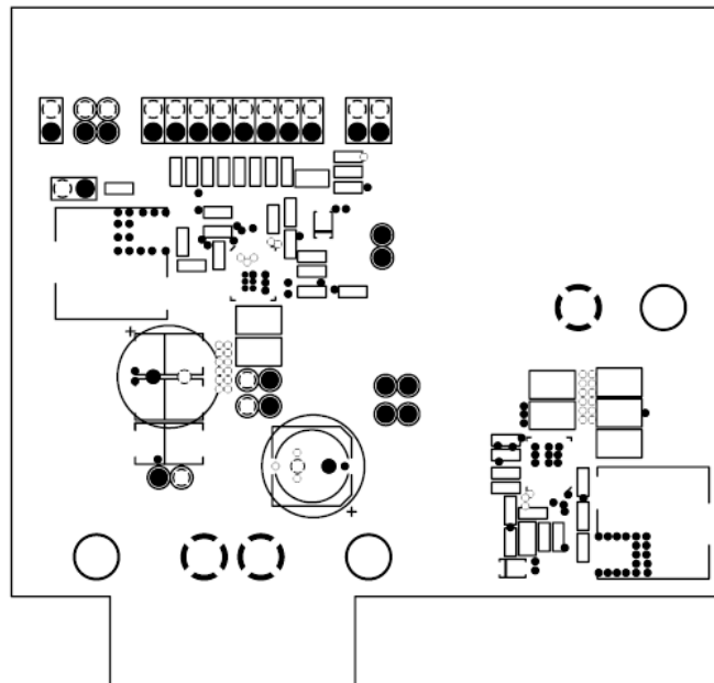
Figure 14. MIC24052 Evaluation Board Mid-Layer 1 (Ground Plane)
