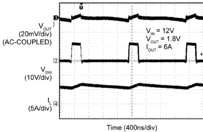
Switching Waveforms
