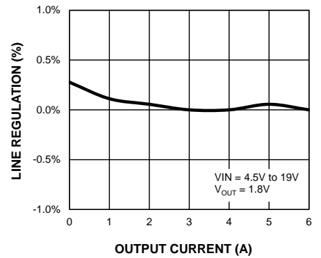
Line Regulation vs. Output Current
