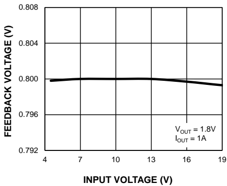
Feedback Voltage vs. Input Voltage
