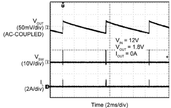
Switching Waveforms
