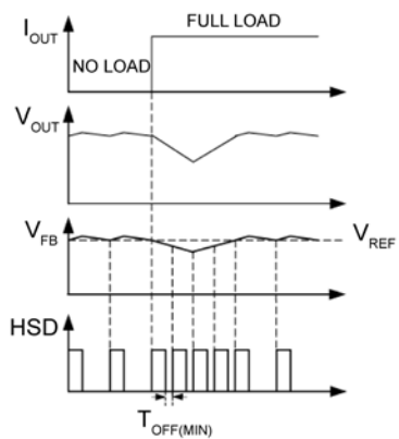
Figure 3. MIC24052 Load Transient Response
