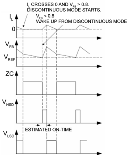
Figure 4. MIC24052 Control Loop Timing (Discontinuous Mode)
