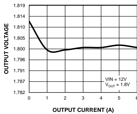
Output Voltage vs. Output Current
