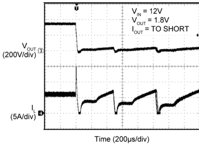
Short Circuit
