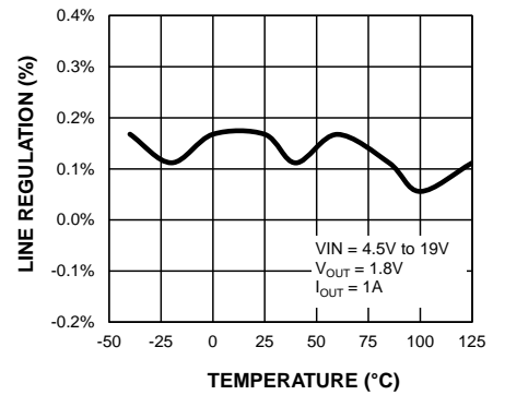
Line Regulation vs. Temperature
