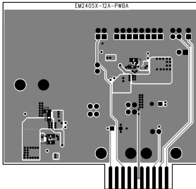
Figure 16. MIC24052 Evaluation Board Bottom Layer
