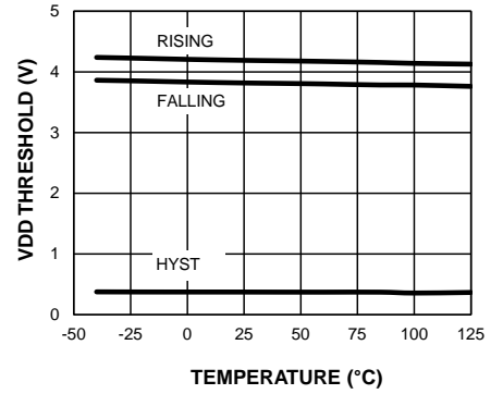
VDD UVLO Threshold vs. Temperature
