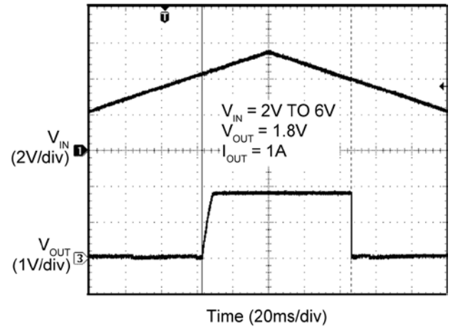
V_{IN} UVLO Threshold
