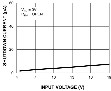
VIN Shutdown Current vs. Input Voltage
