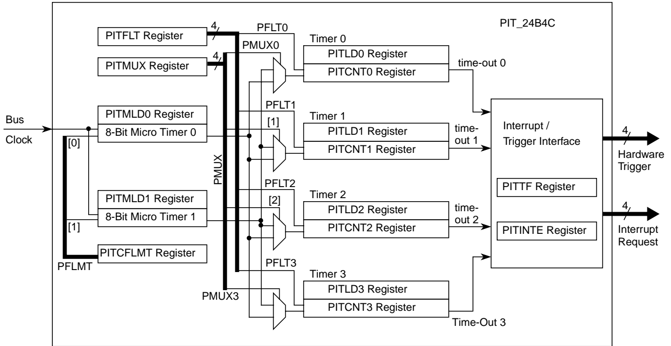
Figure 13-19. PIT Detailed Block Diagram
