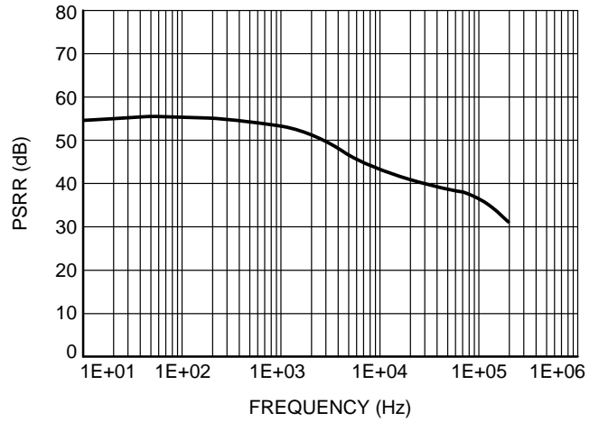
Figure 12. PSRR @ 10 mA
