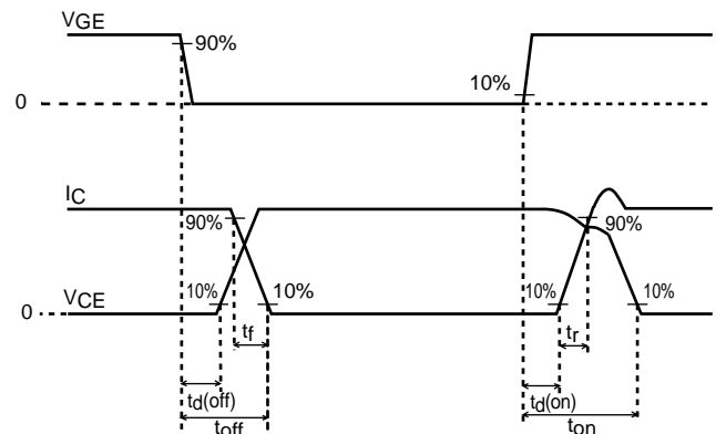
Fig.2 Timing Chart
