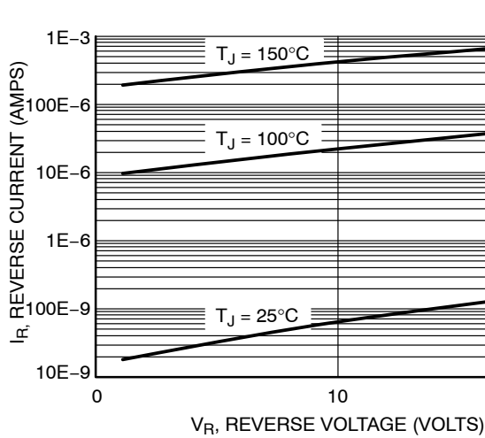
Figure 13. Typical Reverse Current
