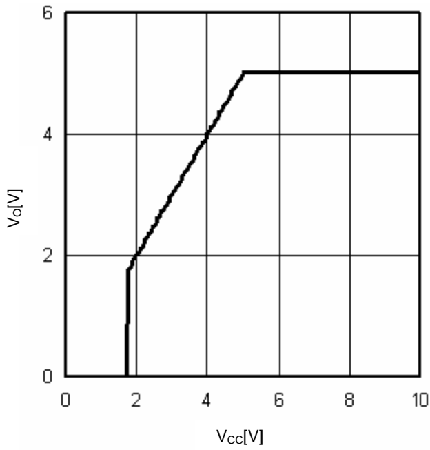
Fig.14 V_{CC}-V_O ( I_o=0mA )
