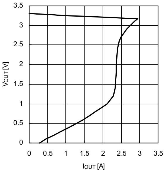
Figure.23 IOUT-VOUT (VIN=3.3V)
