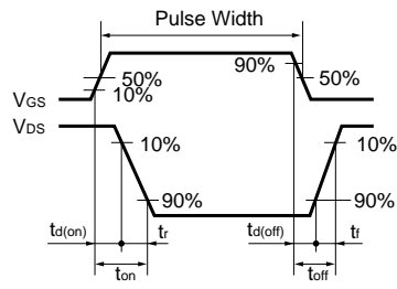
Fig.16 Switching Waveforms
