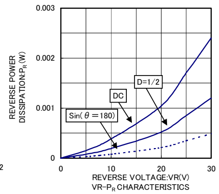
VR-PR CHARACTERISTICS
