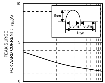
NUMBER OF CYCLES I_{FSM} -CYCLE CHARACTERISTICS
