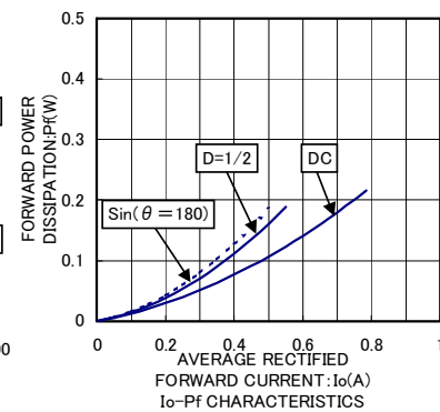
Io-Pf CHARACTERISTICS
