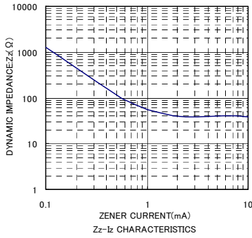
Zz-Iz CHARACTERISTICS
