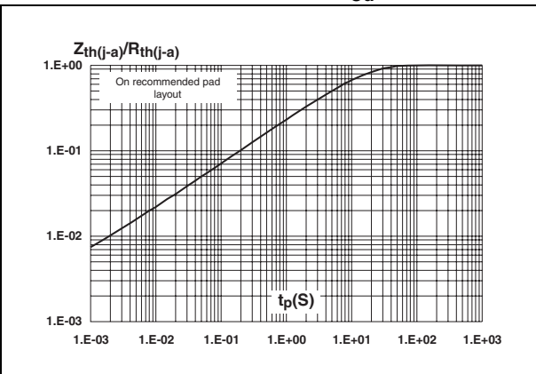
Figure 7. Relative variation of thermal impedance junction to ambient versus pulse duration (printed circuit board FR4, S CU = 1 cm 2 )
