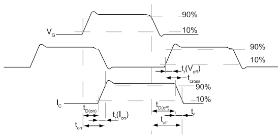
Figure 31: Switching waveform
