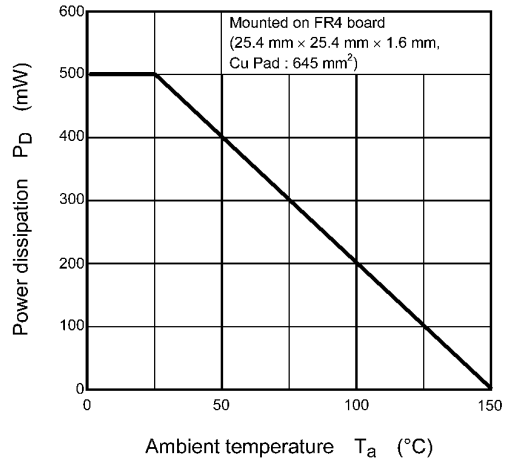
Fig. 8.14 P_D - T_a
