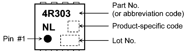
Fig. 7.1 Marking
