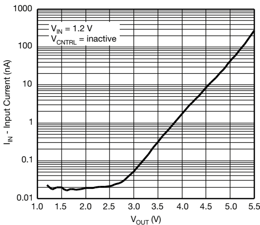
Figure 15 - Reverse Blocking Current vs. Output Voltage
