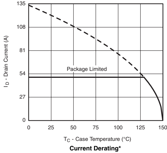
Current Derating*
