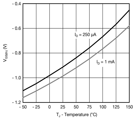
Threshold Voltage
